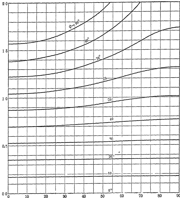
FIG 3 The Elliptic Integral F(\theta, \phi) k = \sin \theta \longrightarrow \theta
